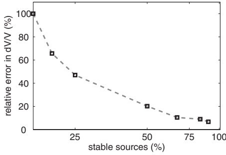
FIG. 11. Relative error in the estimation of \varepsilon=dV/V , versus the ratio of unchanged-to-total amount of noise sources (x-axis in logarithmic scale).
